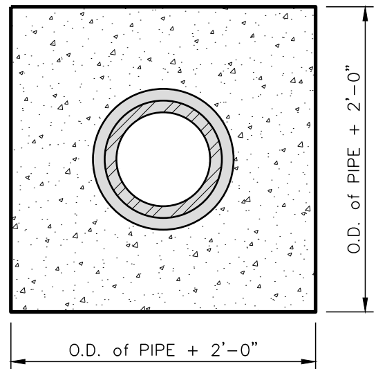
TRANSVERSE SECTION
