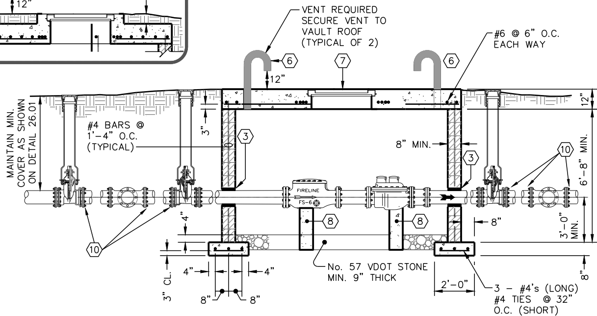
SECTION A
