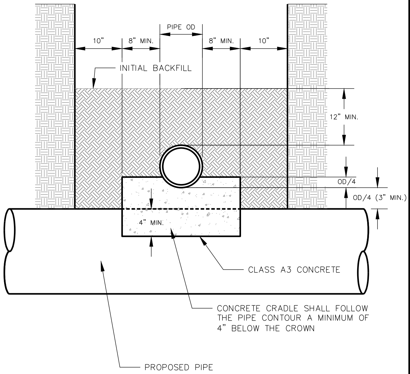
CRADLE DETAIL
