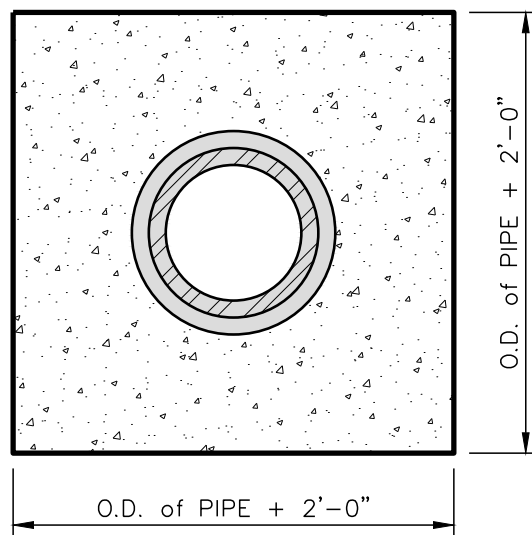
TRANSVERSE SECTION
