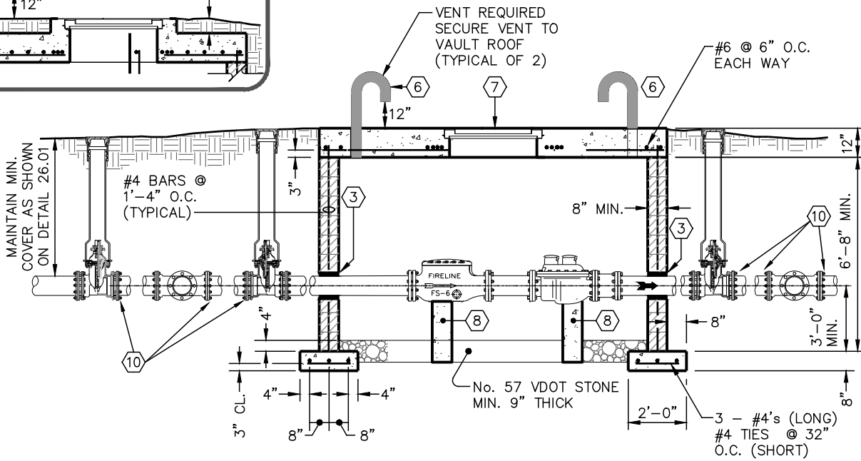
SECTION A
